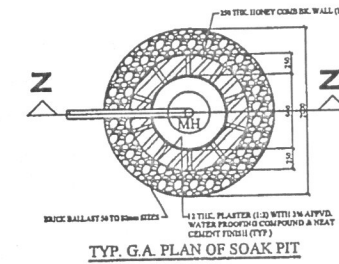
TYP. G.A. PLAN OF SOAK PIT
