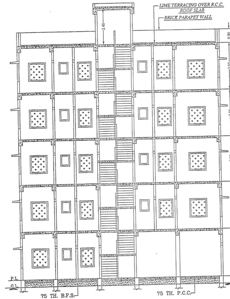
SECTION ON - 'BB'
