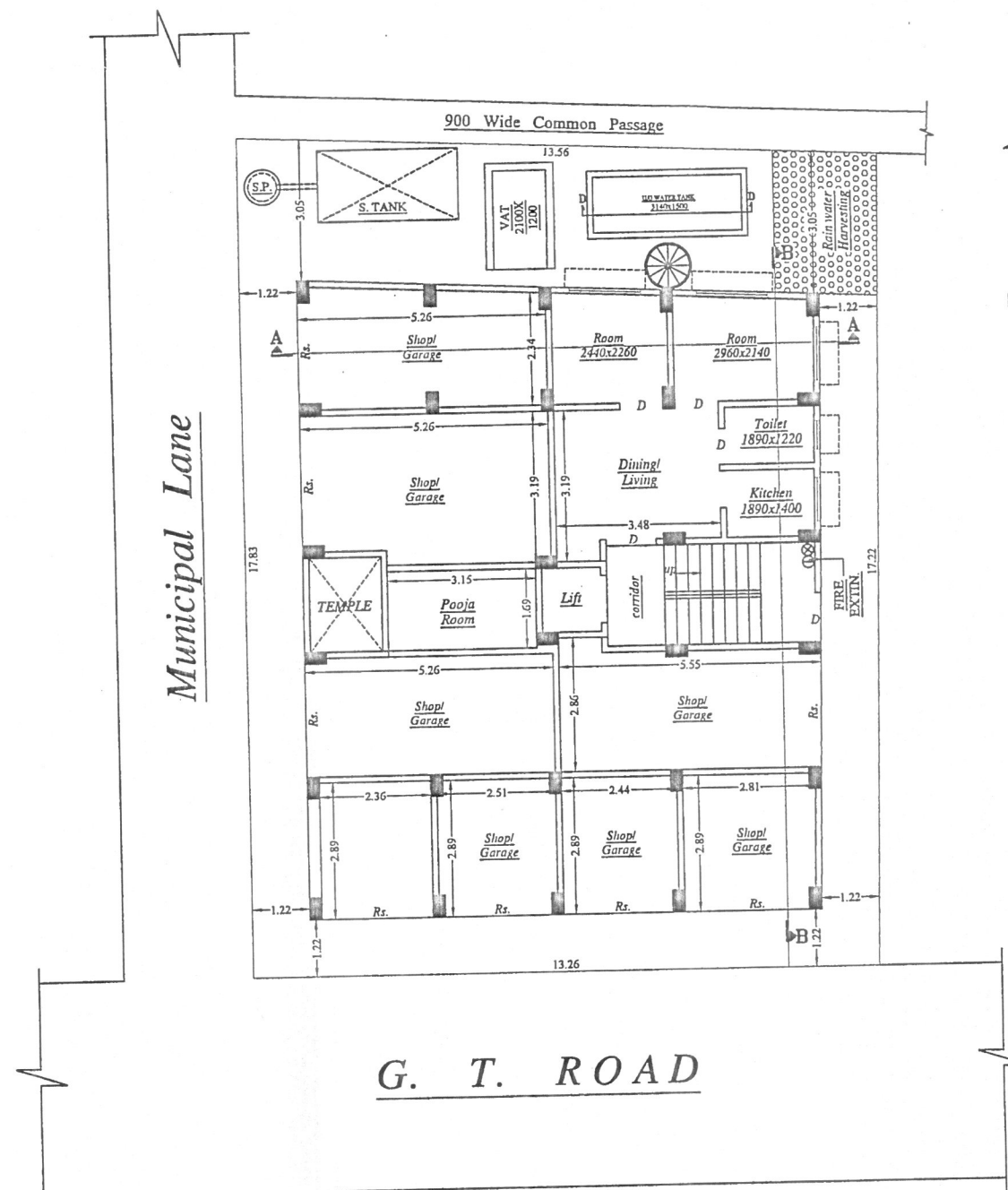
FLOOR-GROUND
