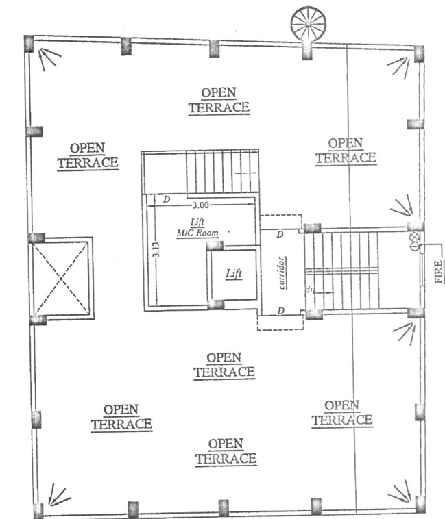
FLOOR-TERRACE
